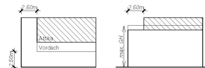
Attikageschoss
